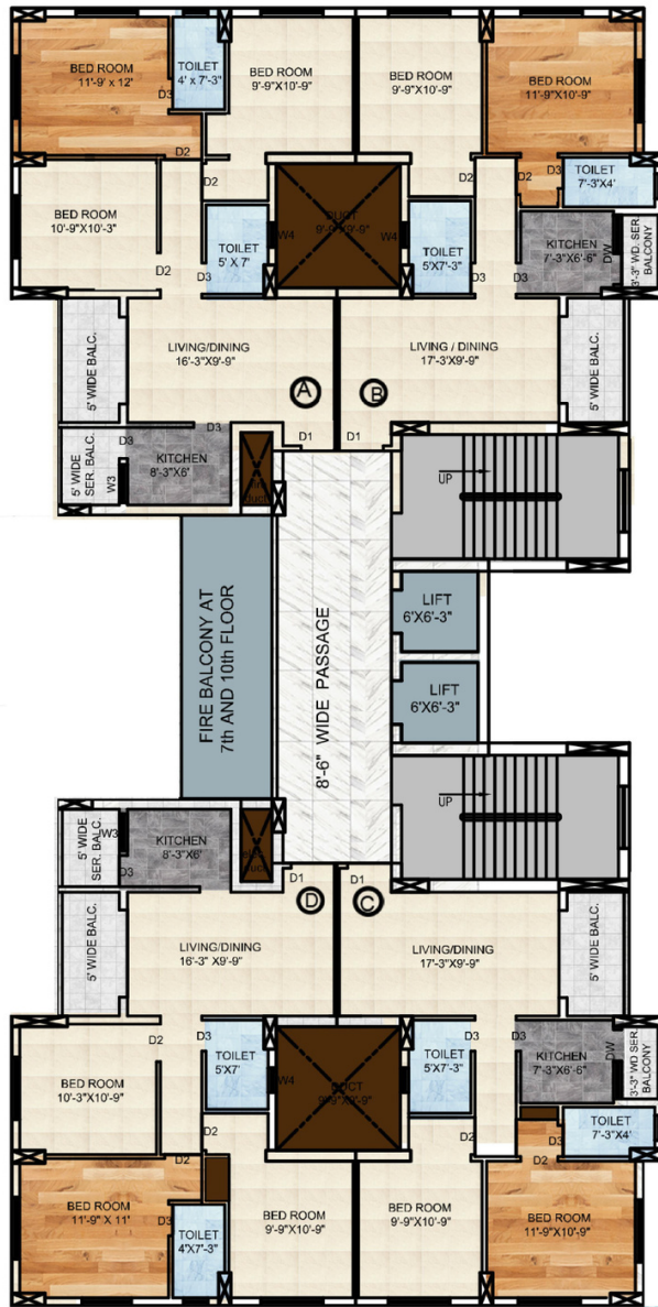
BLOCK B TYPICAL FLOOR PLAN
