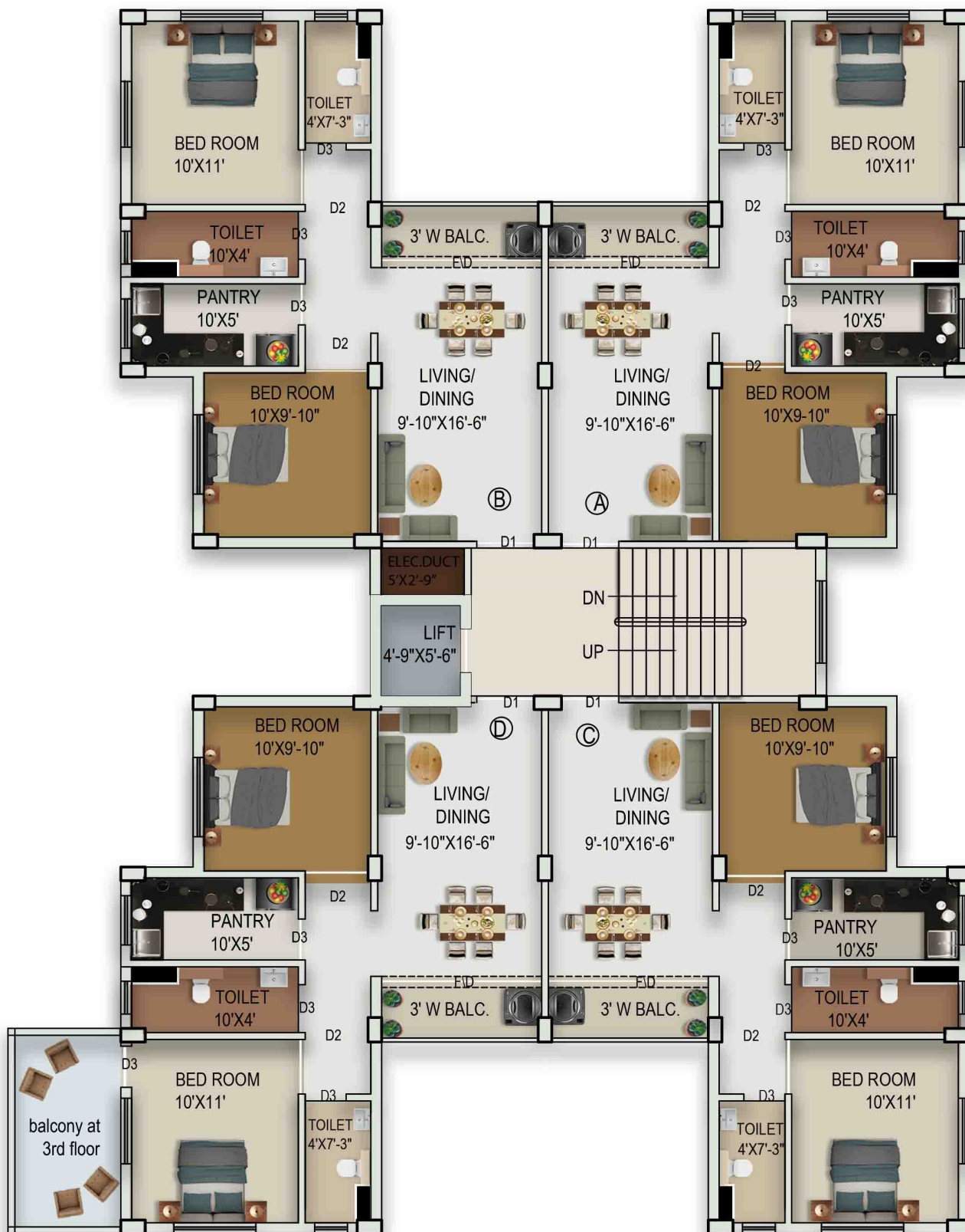
3RD FLOOR PLAN BLOCK 5
